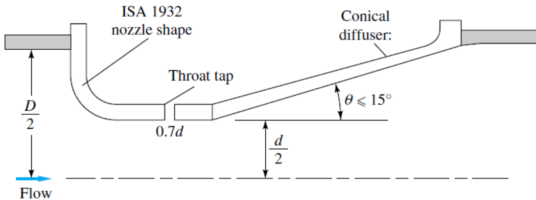
Figure 2.2.3. International standard shapes for venturi nozzle
